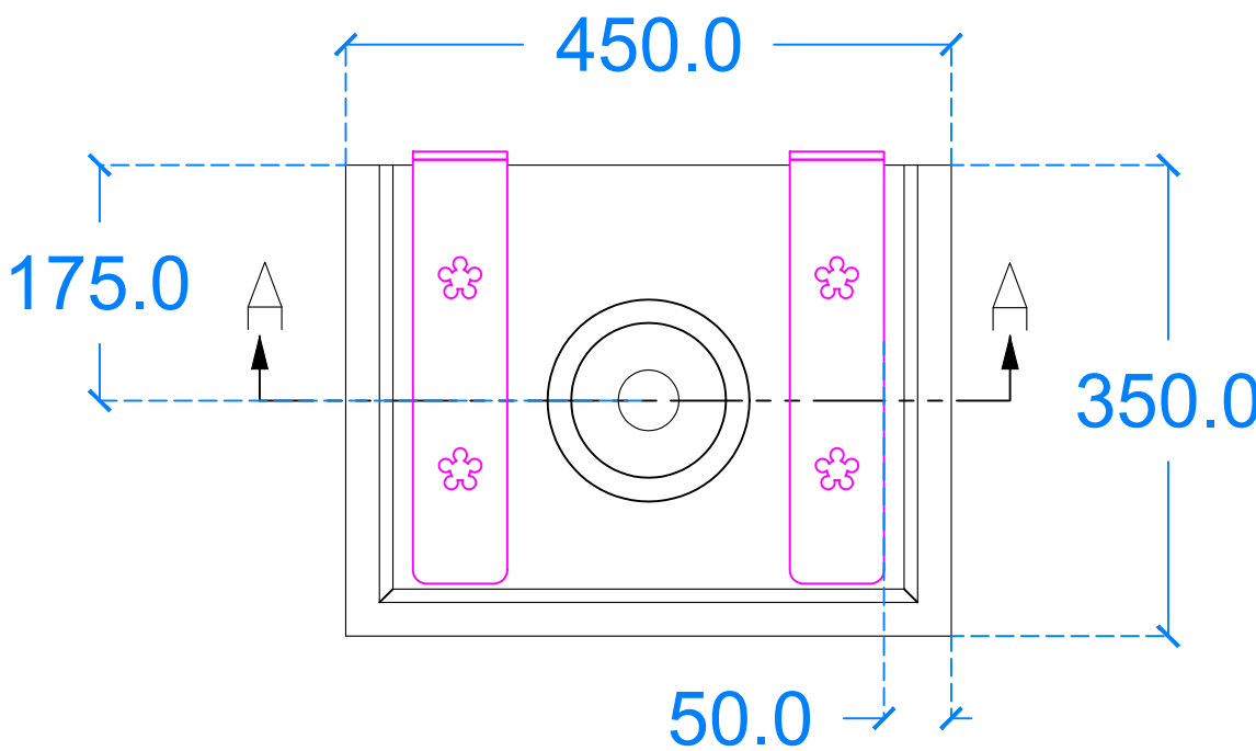
Underside View
