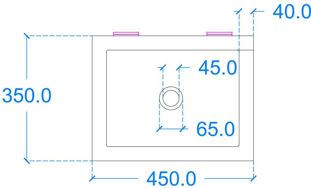
Plan View
